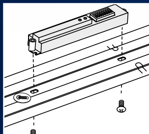
Microwave Sensor Installation
