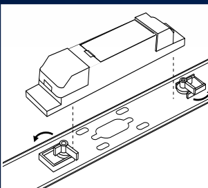
Emergency Pack Installation
